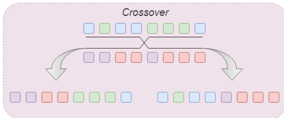
Figure 2.2: Crossover operator overview. The chromosomes of two the parents are combined into the offspring chromosomes , who inherit characteristics from both parents .
