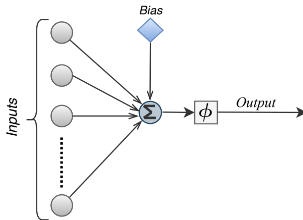
Figure 2.5: Neuron Representation
