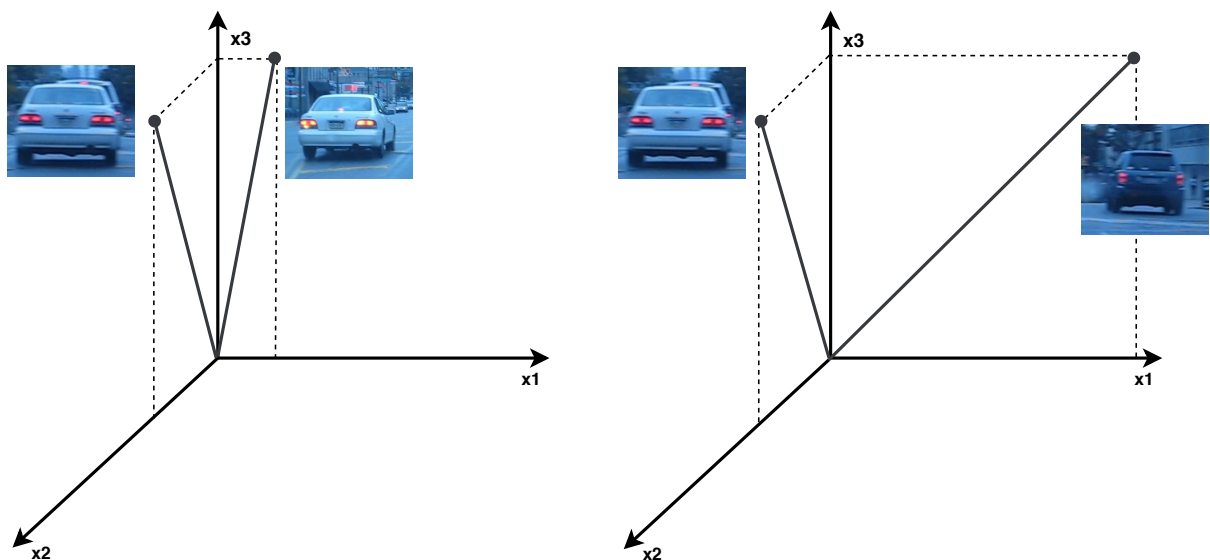
Figure 2.12: Points encoding the respective images in a 3-dimensional space. Notice that very similar images are placed close from each other, and different ones are localized far apart.
