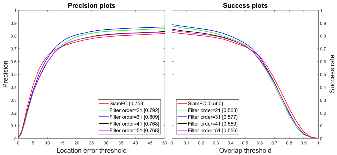
Figure 5.3: Analysis of the filter order of the filter bank used by Short Term Memory . The respective AUCs are shown in the legend between brackets.
