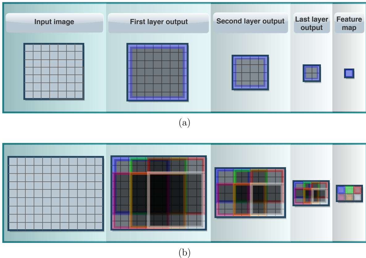
Figure 2.11: Evaluation process of an FCNN (a) Evaluation of an image of atomic size. Its output feature map is reduced to a single feature vector. In this case, the output resembles the evaluation of an ordinary CNN. (b) Evaluation of an image greater than atomic image. In this case, there is a feature map whose size is given by the equation 2.11.
