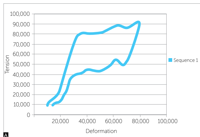
Figure 2 - A) Curve initially obtained on Microsoft Excel. B) Mechanical properties obtained from the curves.
