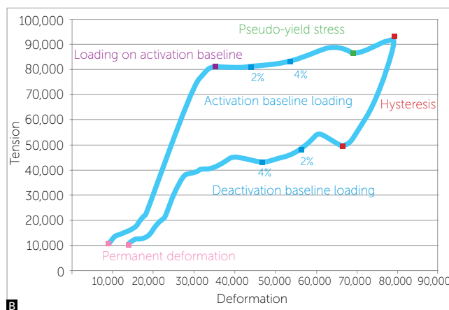
Figure 2 - A) Curve initially obtained on Microsoft Excel. B) Mechanical properties obtained from the curves.
